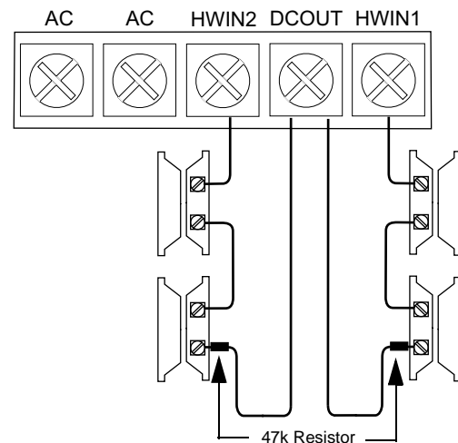
Figure 7. Connecting Normally Closed Hardwire Reed Switches
